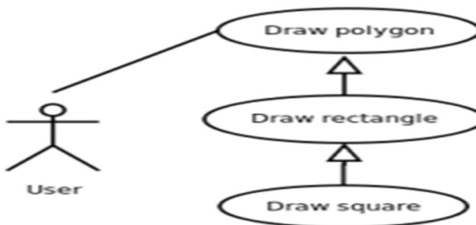
Figure - 04: Generalization relationship among use cases
